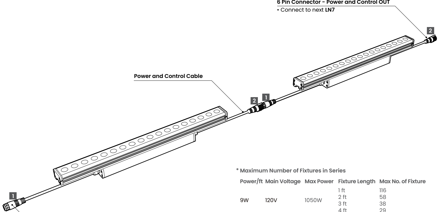
6 Pin Connector - Power and Control IN
