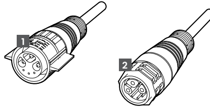
1 6 Pin Connector – Power and Data IN
