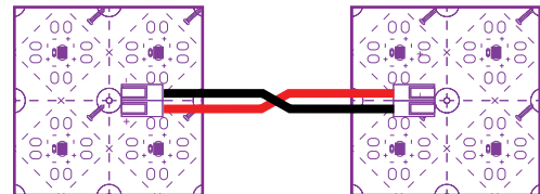
Sheet to Sheet Connection Power Cable
