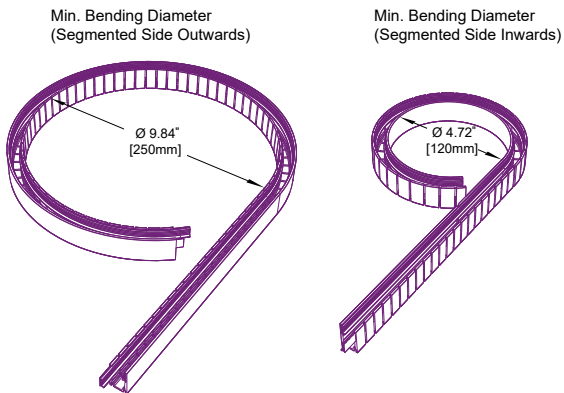
Figure 15 Flexible Mounting Channel
