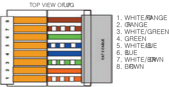
RJ45 CONNECTOR A (LEFT HAND) – DIMMING
