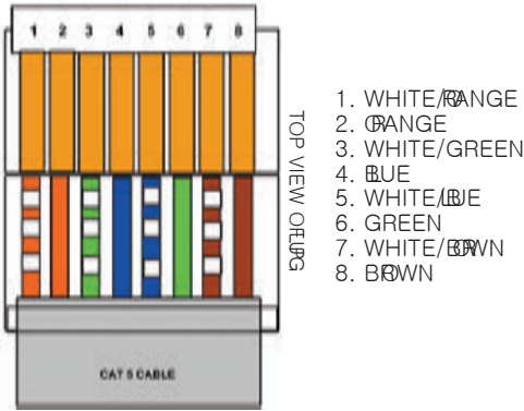
RJ45CONNECTOR A (LEFT HAND) – DIMMING
