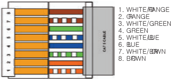
RJ45 – CLIP DOWN, PINS UP TOP VIEW OF RJ45
